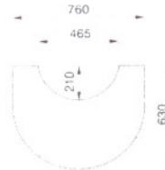
Contura 500 (not 520T) & 600 (not 685, 690), short model
